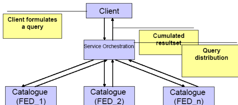
Figure 26: Implementing distributed search
