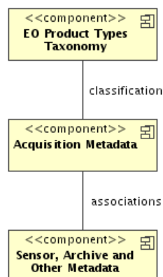
Figure 8: EO Products Mapping Schema Structure
