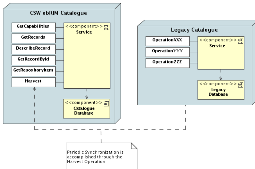
Figure 25: Replication Architecture
