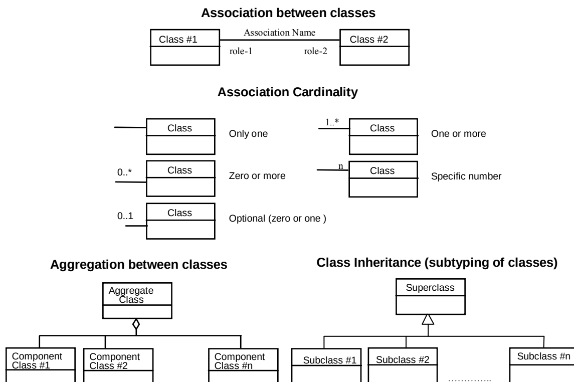
Figure 1: UML notations
