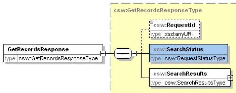
Figure 20: CSW-discovery.xsd (2.0.2) GetRecordsResponse complex type
